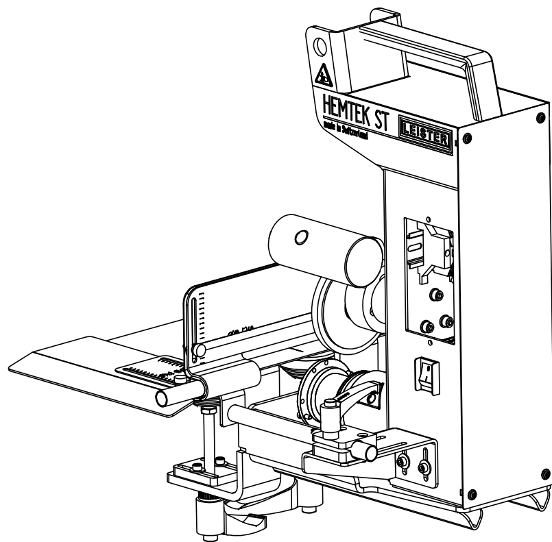
Spare Parts Sheet 2
